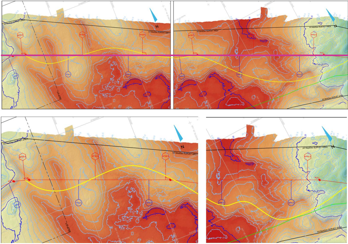
Plate 4.2 Example of micro-routing to link the deepest area of the route corridor (yellow), as opposed to the surveyed Route Position Line (RPL) shown in red with the Kilometre Posts.
